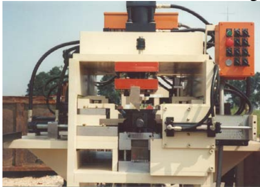
Roll form a tube and form an air tight seam from a flat blank
